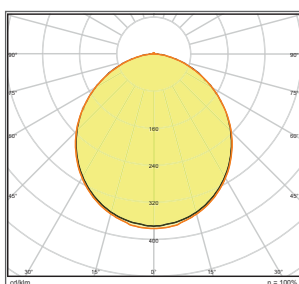
DL SLIM DN 210 18W 6.500K
